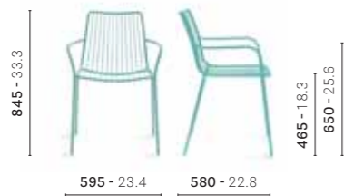
3656 Steel armchair, high backrest
